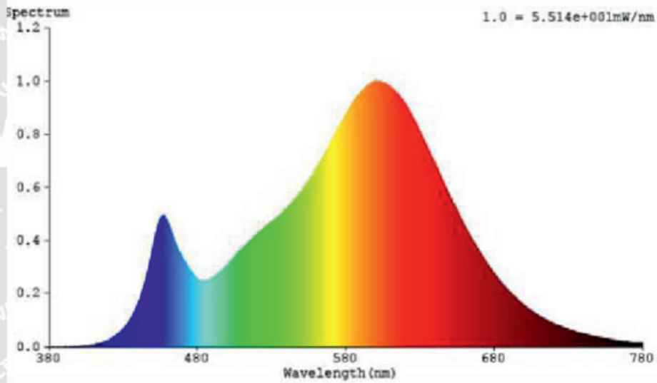
Model: C12653PO (3000K)
