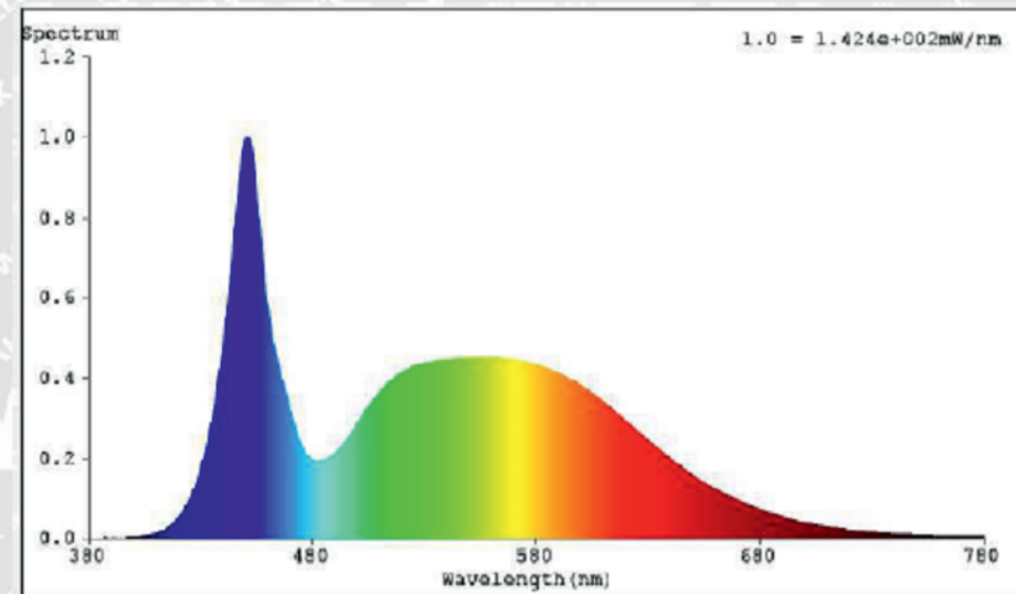
Model: C12653PO (6500K)
