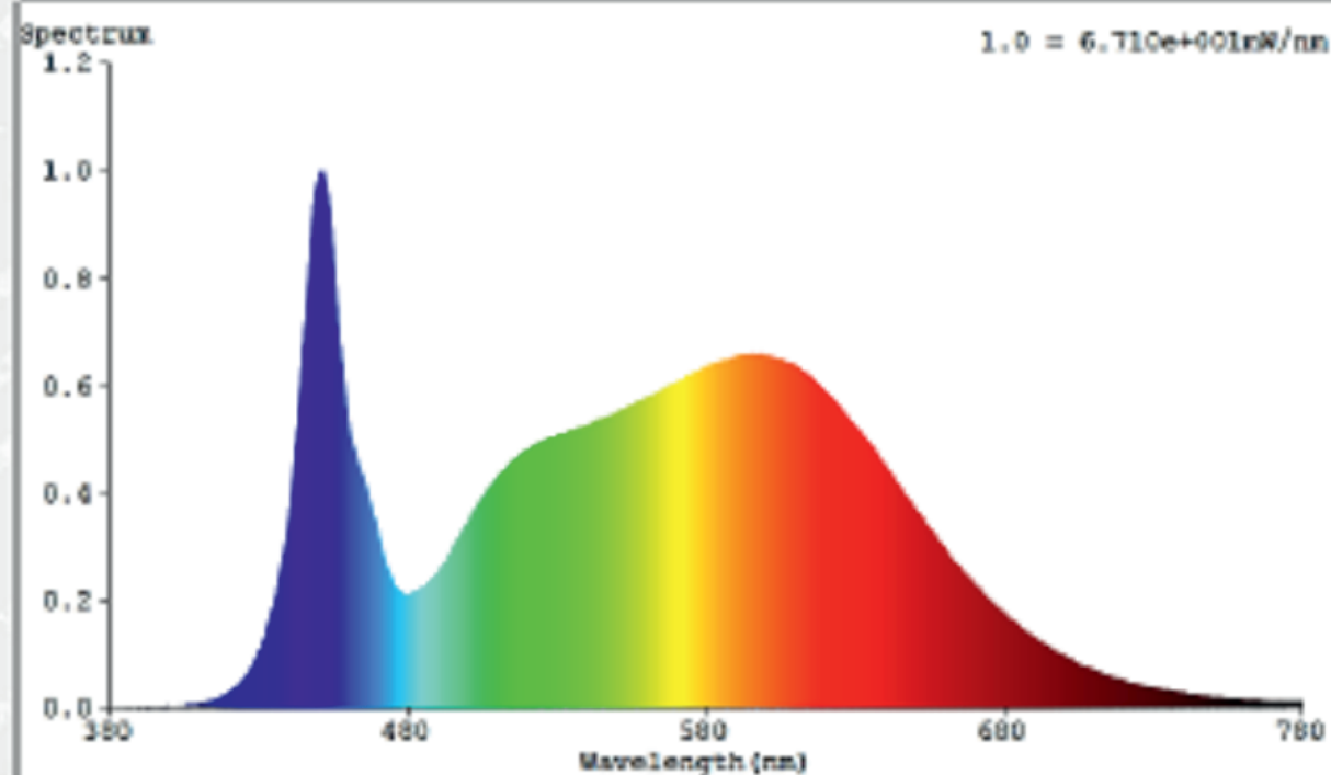
Model: LED Module of CC332470-D (CC3322470) (4000K)
