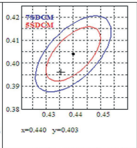
SDCM=3.4 Color Difference Chart
