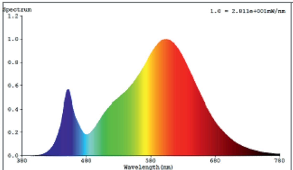
Model: LED Module of CC331640-D (CC3321640) (4000K)
